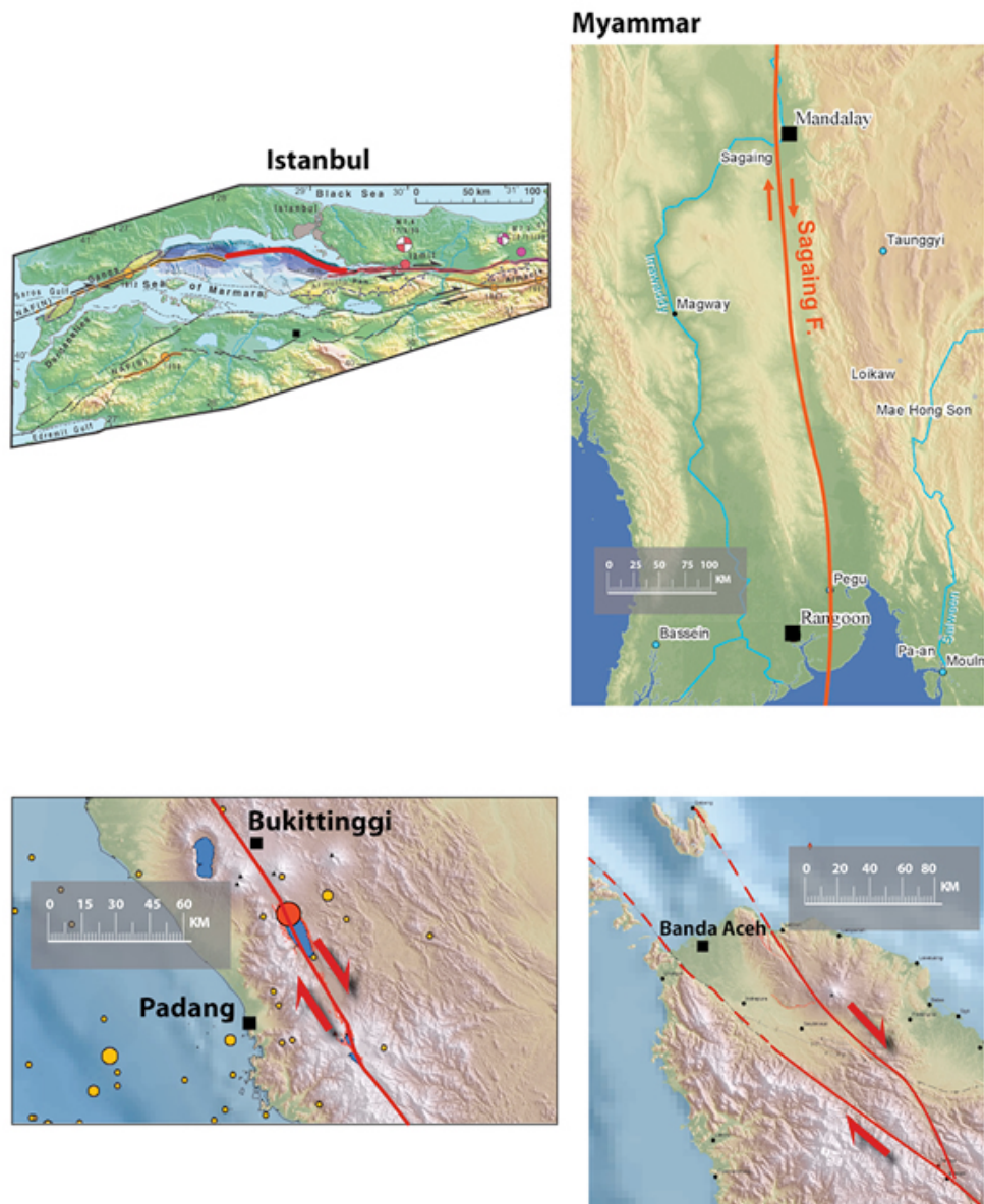
Figure 2: CITIES WITH SIMILAR SEISMIC SITUATIONS
